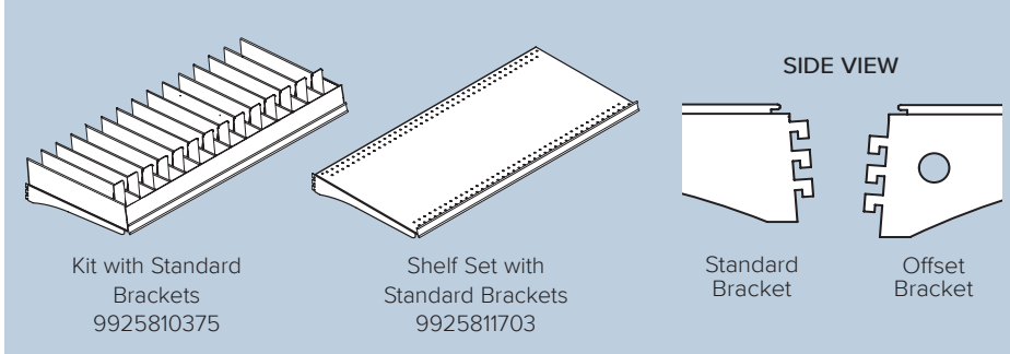
Lozier Shelving with Power Zone® Pre-Set™ Self-facing System (left)
